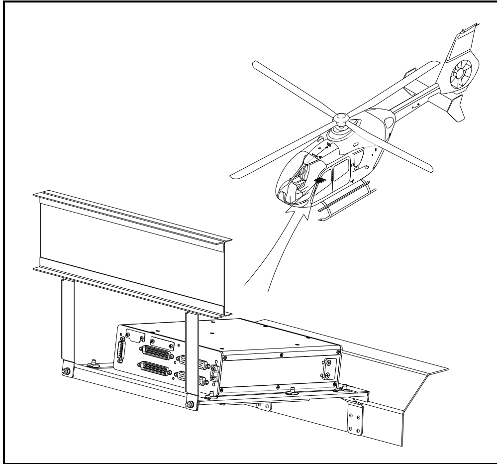
Figure 4 Router Installation
