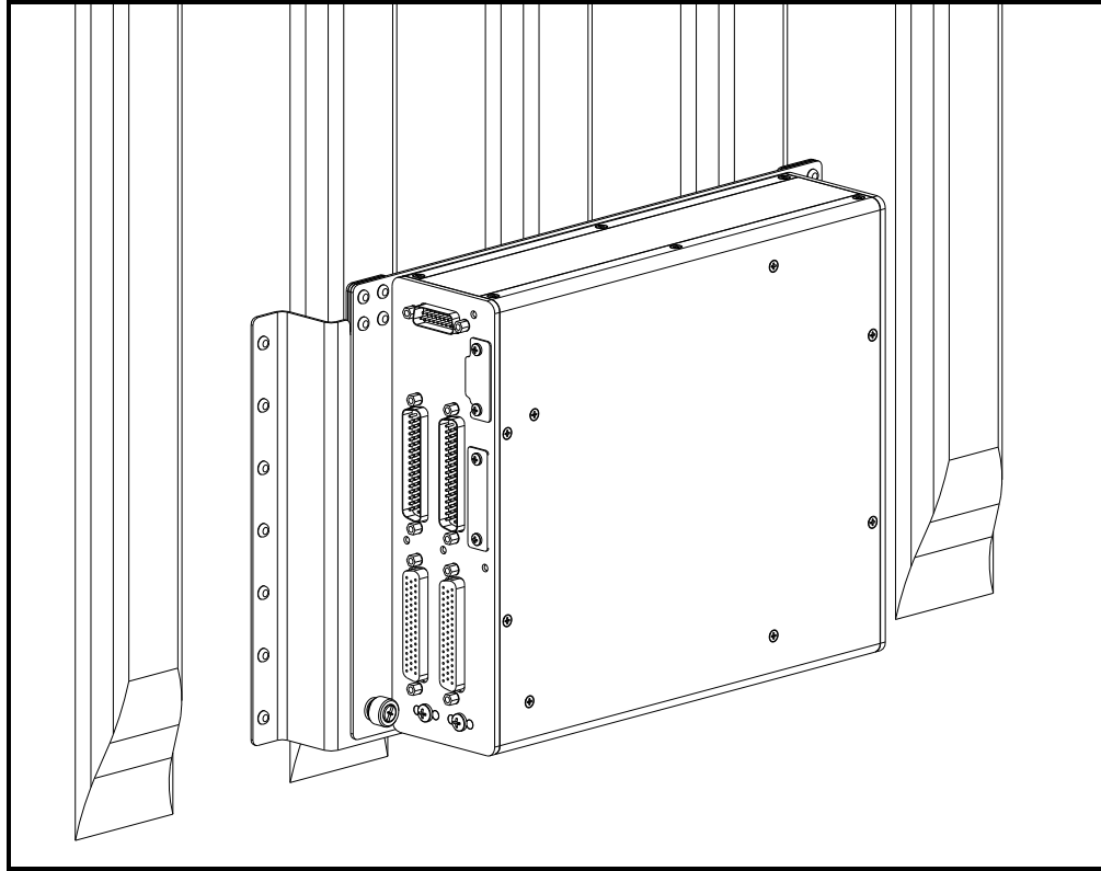
Router Installation in Aft Baggage Compartment
