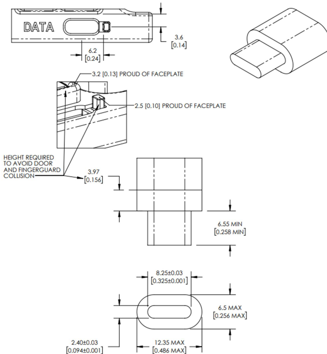
Figure 16: USB Drive Mechanical Requirements
